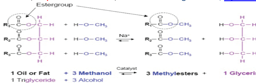
Fig 4 Transesterification of oil and fat
