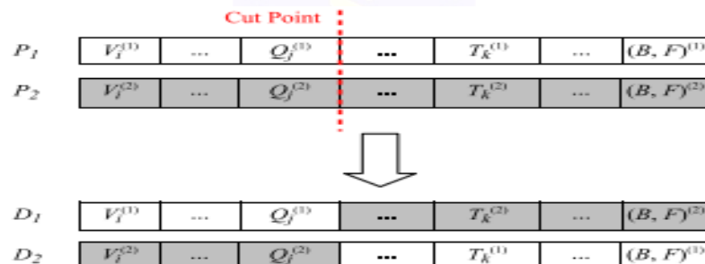
Fig. 1. One-point crossover'
