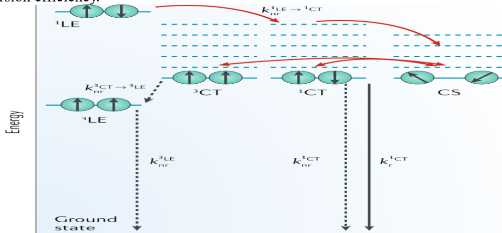
Figure: Charge-transfer electronic states in organic solar cells
