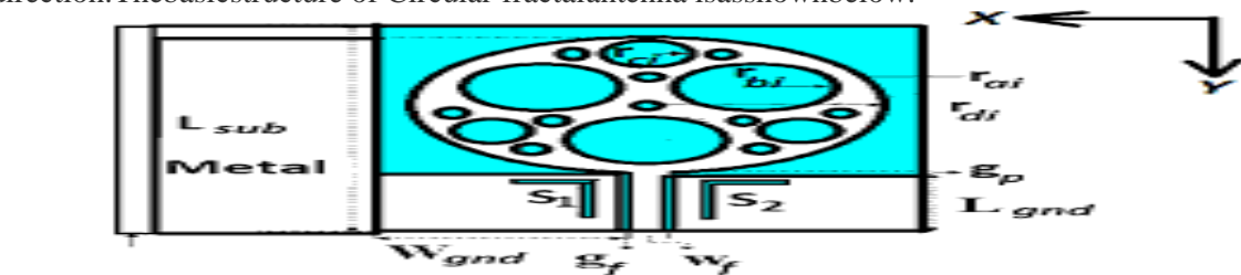
Fig.1 Circular Fractal Antenna structure
