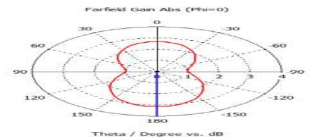
Fig.3(b) radiation pattern for Circular Fractal Antenna
