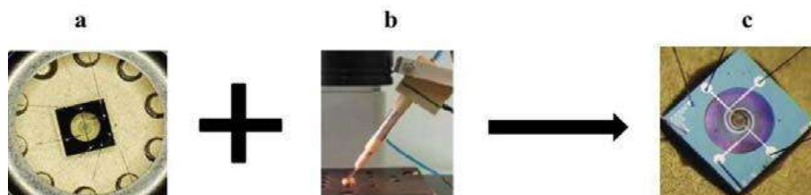
Figure 4. Process of integration of nanoparticles \text{SnO}_2 on the optimized microhotplate. Then, in order to maintain its 20-nanometer size, the drop has been gently and thoroughly oxidised in situ using a carefully calibrated temperature profile (empirically determined and applied to our sensitive layers). Without coalescence and cracking, a porous nanosensitive layer (Figure 5) can be created.
