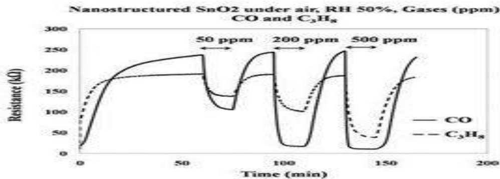
Fig.8. Transient Response to CO and C 3 H 8 at 500°C.
